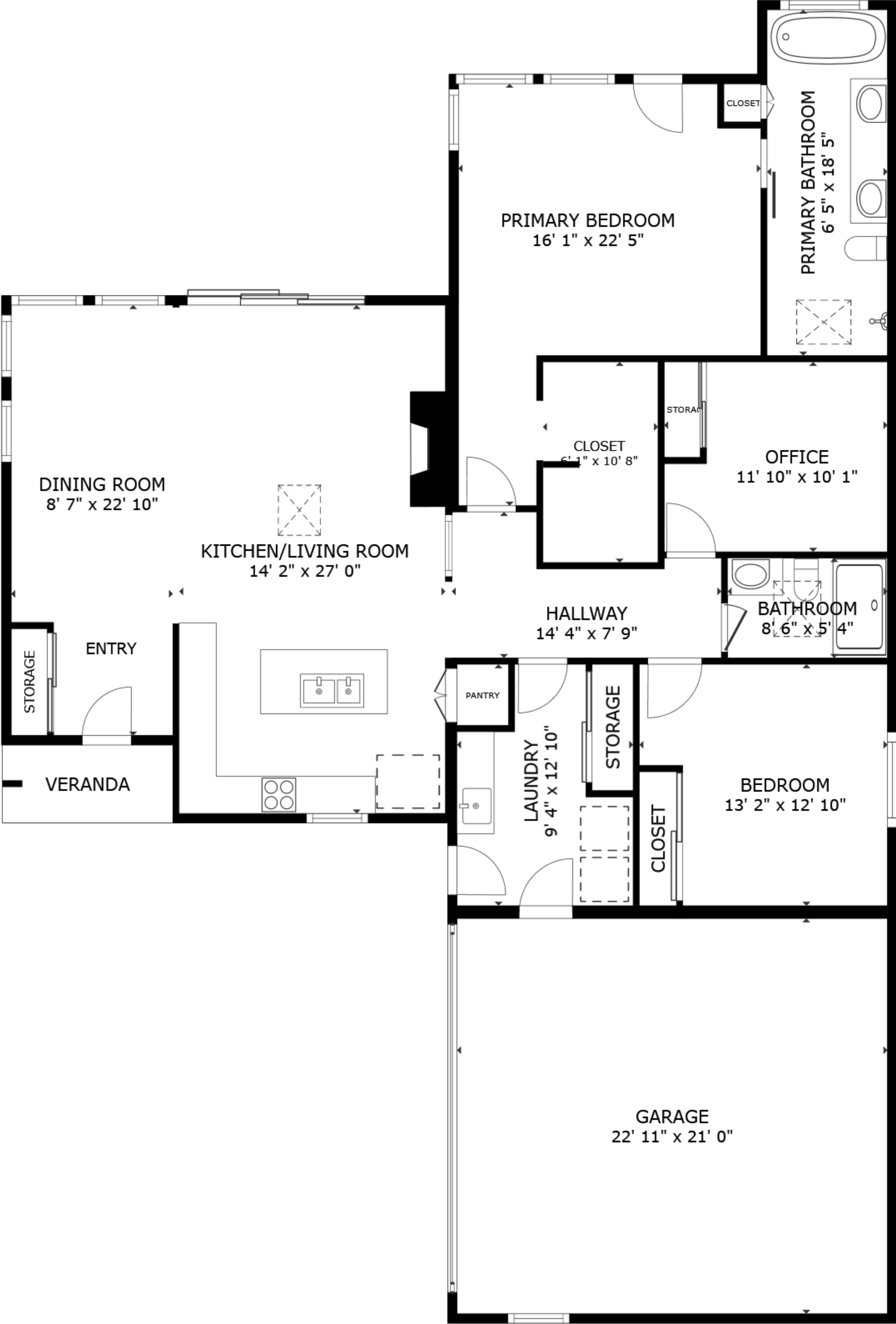
FLOOR PLAN
